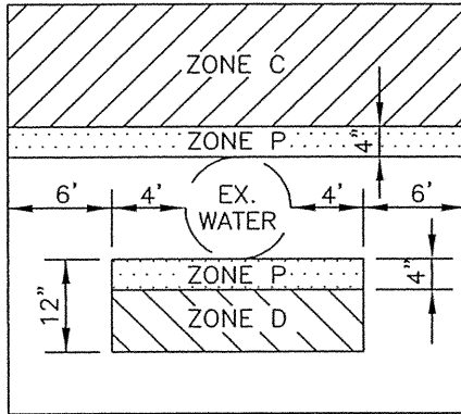
PERPENDICULAR CONSTRUCTION
